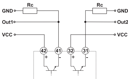
Fig. 26 Static outputs, VCC reference
